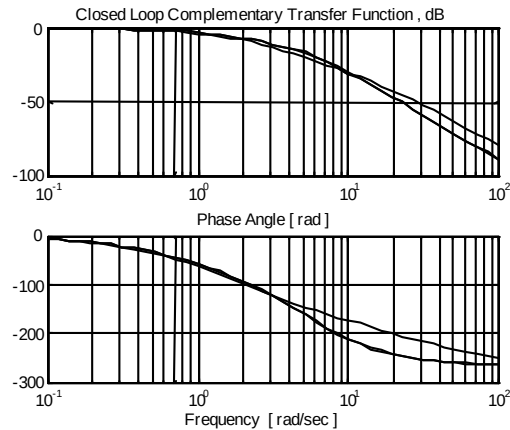
Figure 5. The Complementary Sensitivity of the Closed Loop Control System Q_1 – dotted ; Q_2 – dash-dot ; Q_3 – solid
