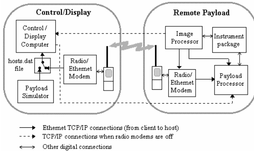
Picture 4. System Functional Diagram
